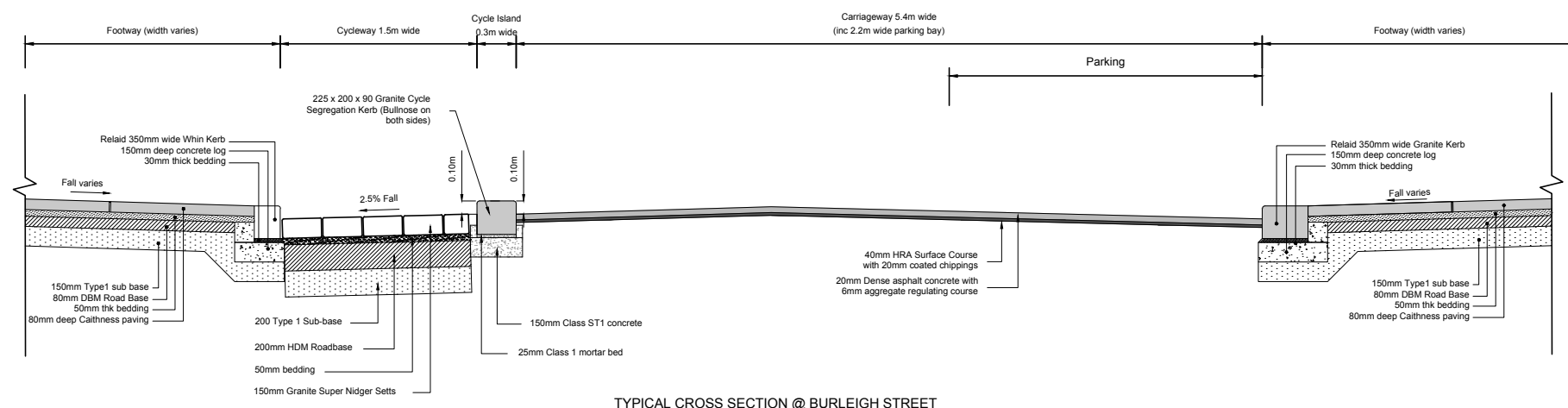
TYPICAL CROSS SECTION @ BURLEIGH STREET 1:20
