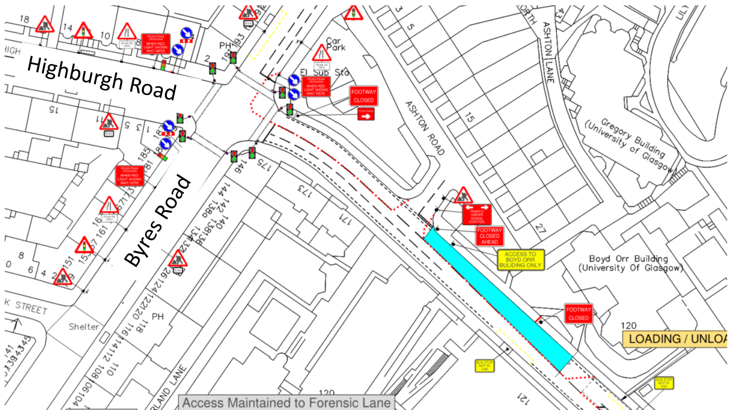
Temporary Traffic Management system at the University Avenue/ Byres Road junction.
